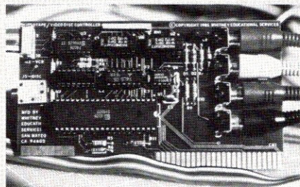
Figure A: The Whitney Supercircuit II CAIV interface card for the Apple II Plus, IIe, and IIGs. It can control VCR and videodisc separately or simultaneously.
