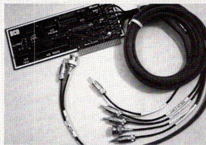
Figure B: BCD's Model 450 CAIV interface for the Apple II Plus and IIe controls a wide variety of VCRs. All the necessary cables are bundled and labeled for easy connection to computer, VCR, and display monitor/TV.
