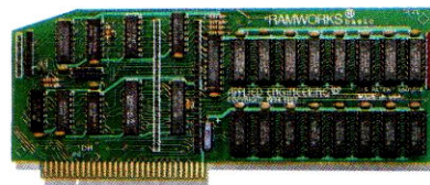
RamWorks basic® expansion board.
